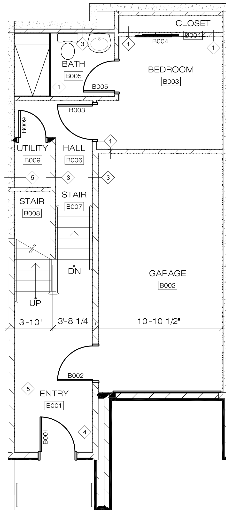
GROUND FLOOR PLAN - UNIT B
